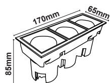
Dimension ( mm )
