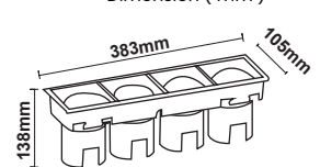
Dimension ( mm )
