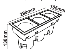
Dimension ( mm )
