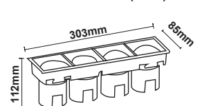
Dimension ( mm )
