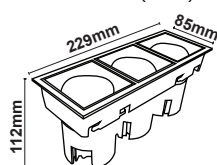
Dimension ( mm )
